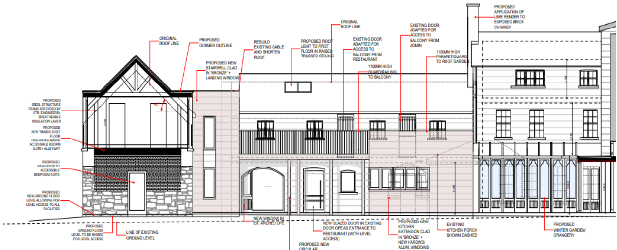
The Forum Mountmellick (The Square) Rear (Side) Elevations
